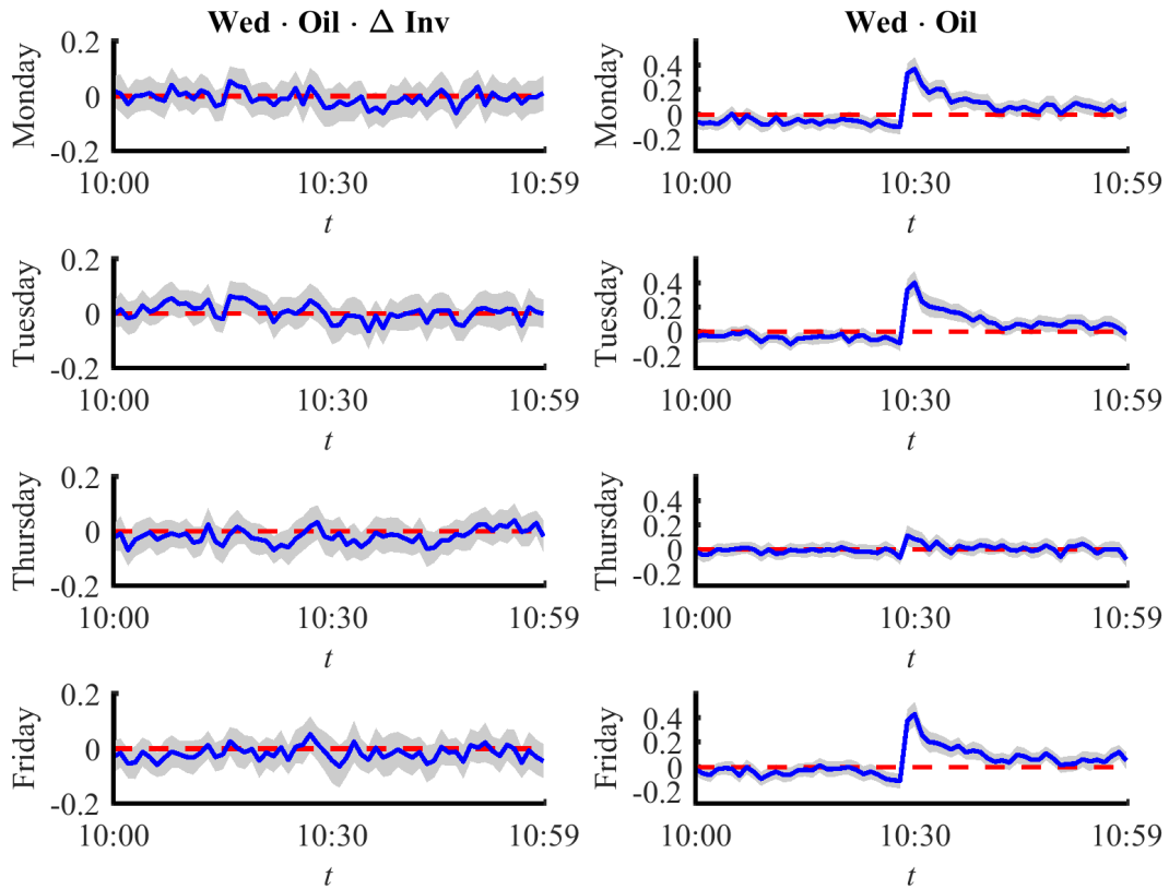
Figure B.6: Different weekday as a control (Volume). This figure plots the estimates (blue line) and their 95 % confidence interval (grey area) of the model described in equation (7), using number of transactions as a dependent variable. I restrict the sample to Wednesdays and another weekday as a control. This control day is Monday in the first row and Tuesday, Thursday and Friday the following rows. I estimate the coefficients independently for every minute exploiting variation across days. The left-hand side plots correspond to \gamma_2 , while the right-hand side ones refers to \gamma_1 . I describe the sample in Section 2. The red dashed line indicates the zero.
