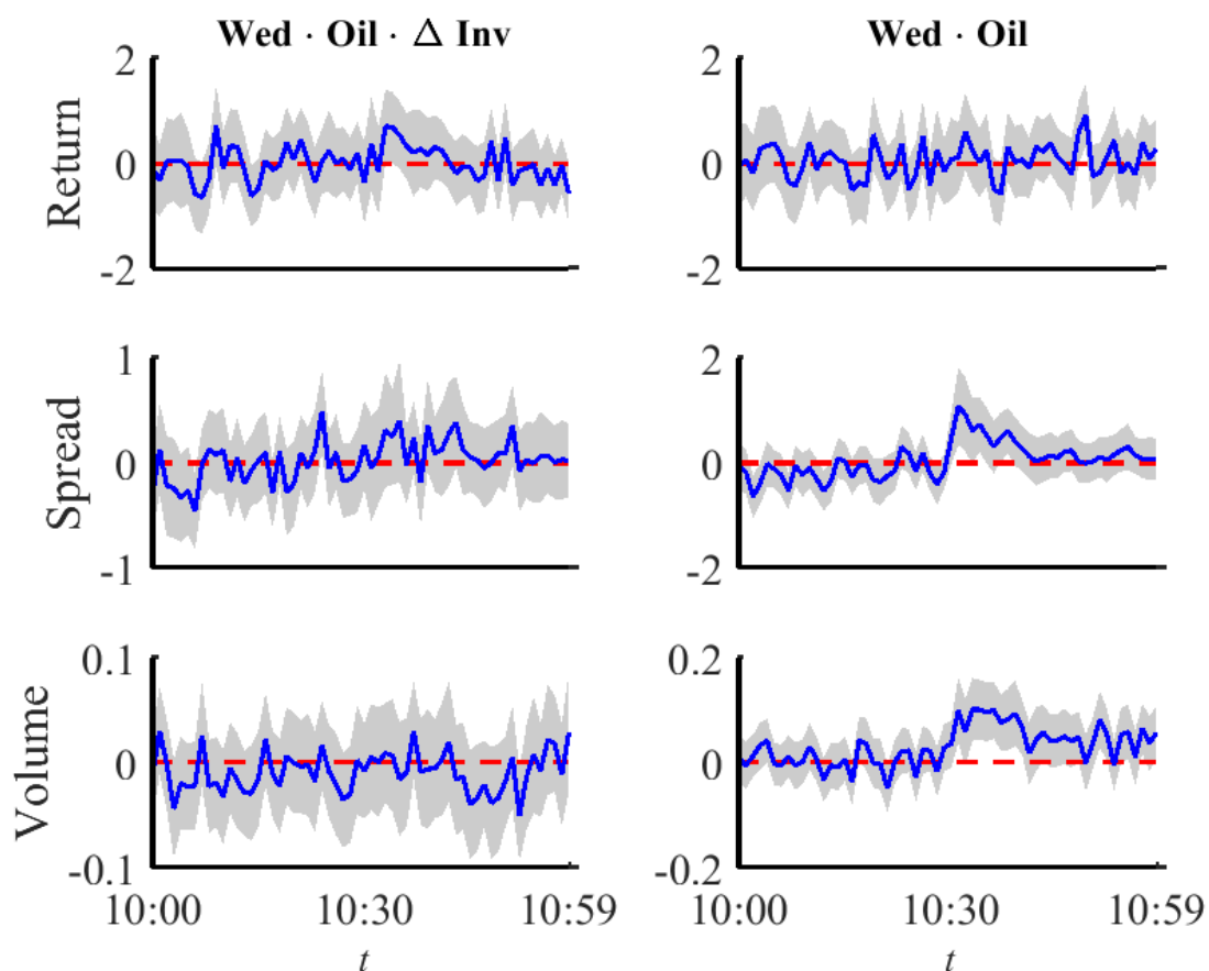
Figure B.9: Estimates Pre-2005. This figure plots the estimates (blue line) and their 95 % confidence interval (grey area) of the model described in equation (4). Each row consider a different dependent variable, from top to bottom: midpoint return, high-low spread, and number of transactions. I estimate the coefficients independently for every minute exploiting variation across days. The left-hand side plots correspond to \gamma_2 , while the right-hand side ones refers to \gamma_1 . I describe the sample in Section 6.4 and I restrict it to observations before year 2004. The red dashed line indicates the zero.
