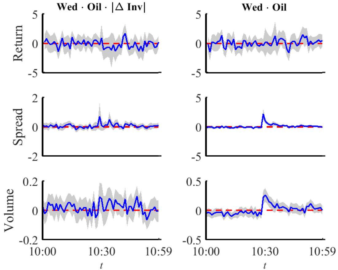
Figure B.3: More Noise Traders. This figure plots the estimates (blue line) and their 95 % confidence interval (grey area) of the model described in equation (7). Each row consider a different dependent variable, from top to bottom: midpoint return, proportional effective bid-ask spread, and number of transactions. I estimate the coefficients independently for every minute exploiting variation across days. The left-hand side plots correspond to \gamma_2 , while the right-hand side ones refers to \gamma_1 . I describe the sample in Section 2. The red dashed line indicates the zero.
