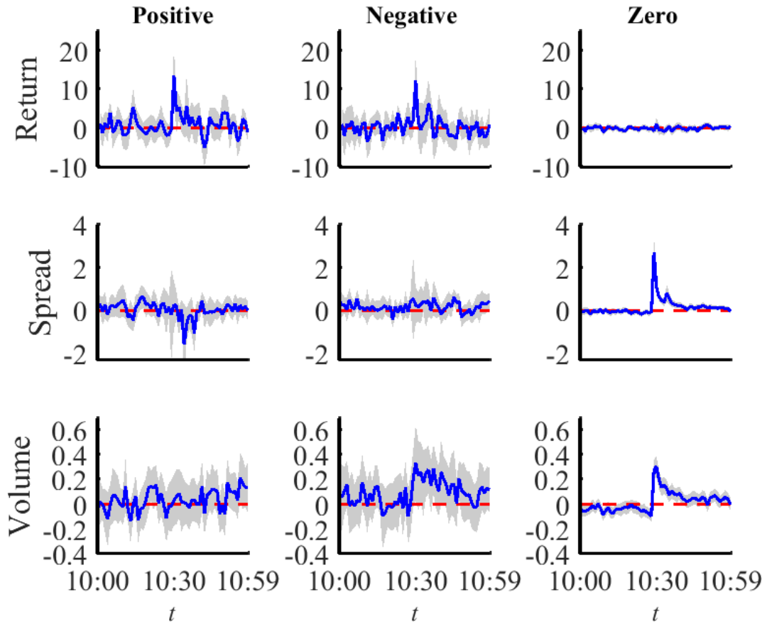
Figure B.2: Binary Specification. This figure plots the estimates (blue line) and their 95 % confidence interval (grey area) of the model described in equation (6) Each row consider a different dependent variable, from top to bottom: midpoint return, proportional effective bid-ask spread, and number of transactions. I estimate the coefficients independently for every minute exploiting variation across days. The left-hand side plots correspond to \gamma_2^+ , and the middle ones to \gamma_2^- ; meanwhile, the right-hand side ones refers to \gamma_1 . I describe the sample in Section 2. The red dashed line indicates the zero.
